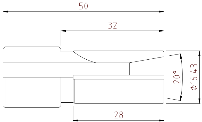
COLLET BODY
