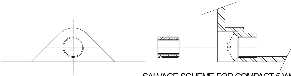
SALVAGE SCHEME FOR COMPACT 5 WORN M8 THREAD IN CARRIAGE
