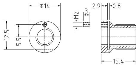
SALVAGE SCHEME FOR COMPACT 5 WORN M8 THREAD IN CARRIAGE & BACKLASH ADJUSTMENT
