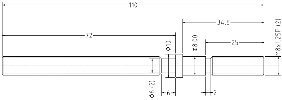
STD FEEDSCREW
