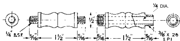
(HEX. NUTS, 1/8" THICK, FITTED EACH END)
