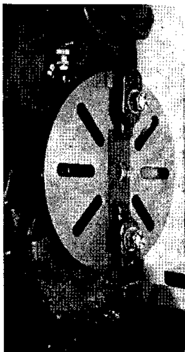
Fig. 15: Set-up for the machining of the curve on the impulse pallet
