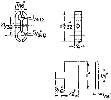
Fig. 18: Clamp block and gathering pawl. Fig. 19 (right) illustrates the contact platform and clamp brass
