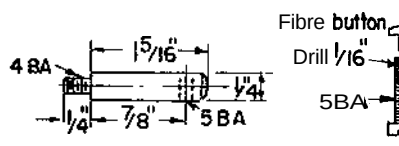
FIG.11 Impulse arm stop brass
