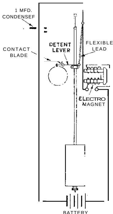
Electrical connections of pendulum mechanism
