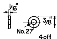
FIG.7. Insulating washer
