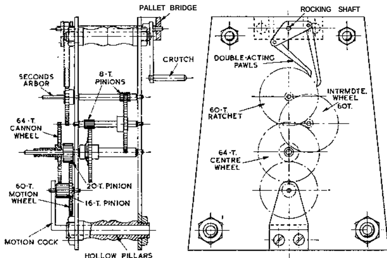
General arrangement of clock movement
