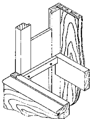
Left, Fig. 9: Detail of strips for shelf
