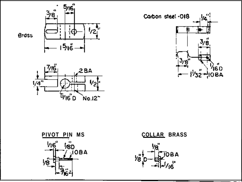
Fig. 18: Clamp block and gathering pawl. Fig. 19 (right) illustrates the contact platform and clamp brass
