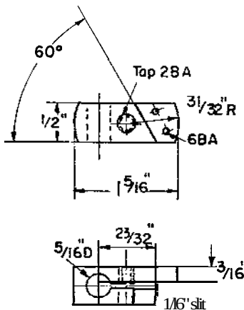
FIG.13 Pendulum clamp block and impulse pallet
