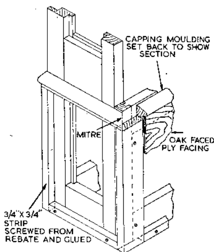
Fig. 7: Constructing the rails for the bottom of the clock case
