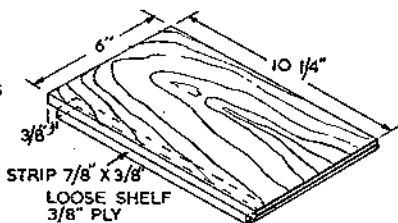
Fig. 11: Loose shelf of \frac{3}{8} in. ply
