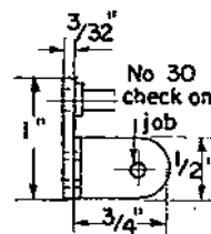
FIG.12 Impulse arm 3/32" brass
