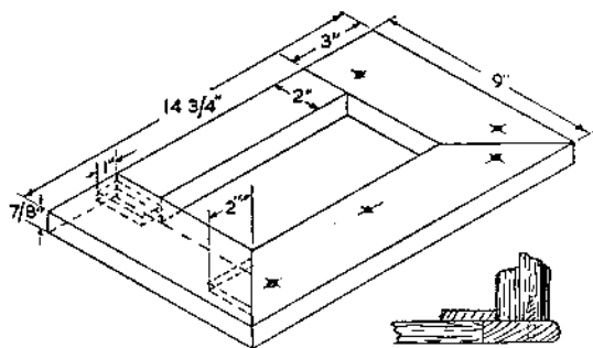
Left, Fig. 8: Base of the clock
