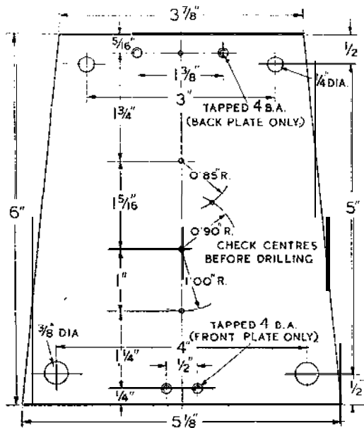
MOTION PLATE 2 OFF BRASS
