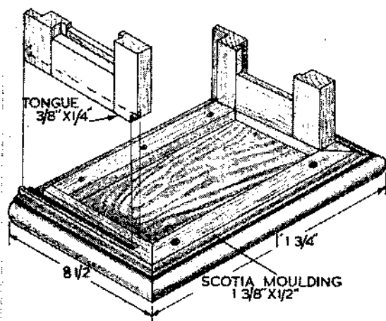
Above, Fig. 6: Details of the separated tongue and the groove joint
