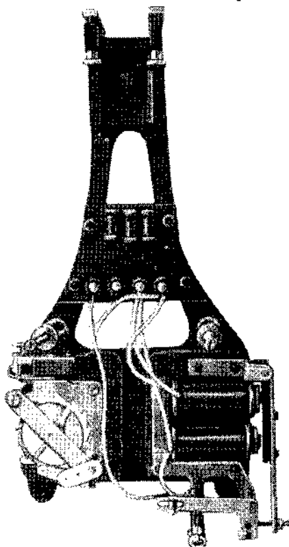
Baseplate of clock with electrical gear, and fitted with Mr Wilding's impulse mechanism.
