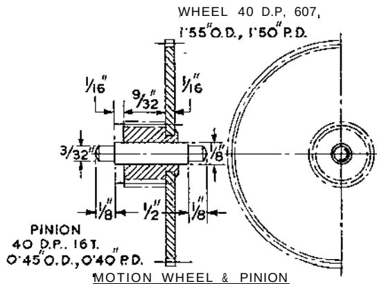
MOTION WHEEL & PINION
