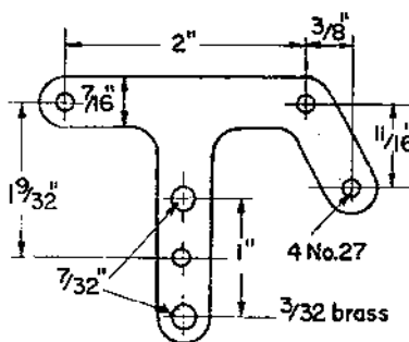
FIG.6 Sub plates for magnet assy.
