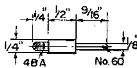
FIG.9 Impulse arm pivot post. MS
