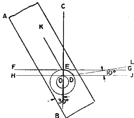
FIG.14 Marking out diagram for impulse pallet. 1 "x1/8" brass strip
