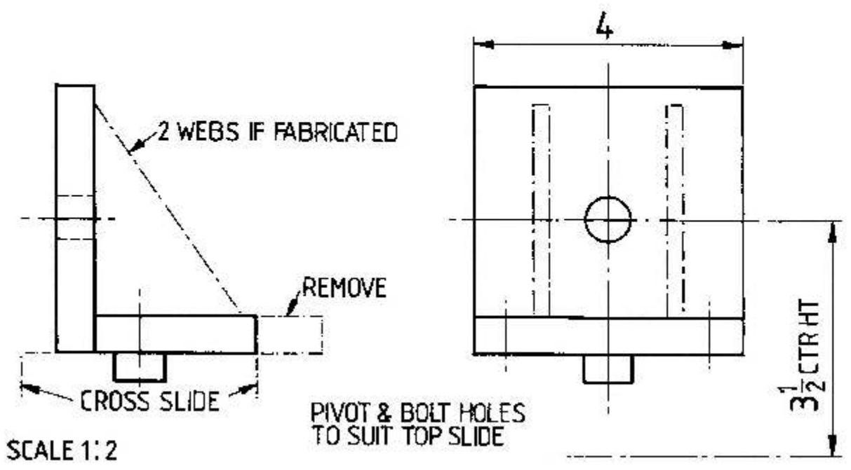
SCALE 1:2 ITEM 2 LATHE MOUNT CAST IRON
