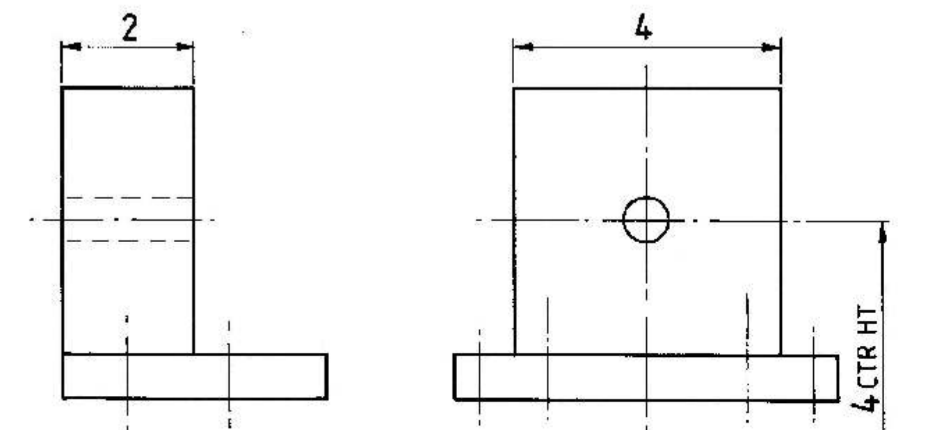
SCALE 1:2 ITEM 4 LATHE MOUNT MILD STEEL
