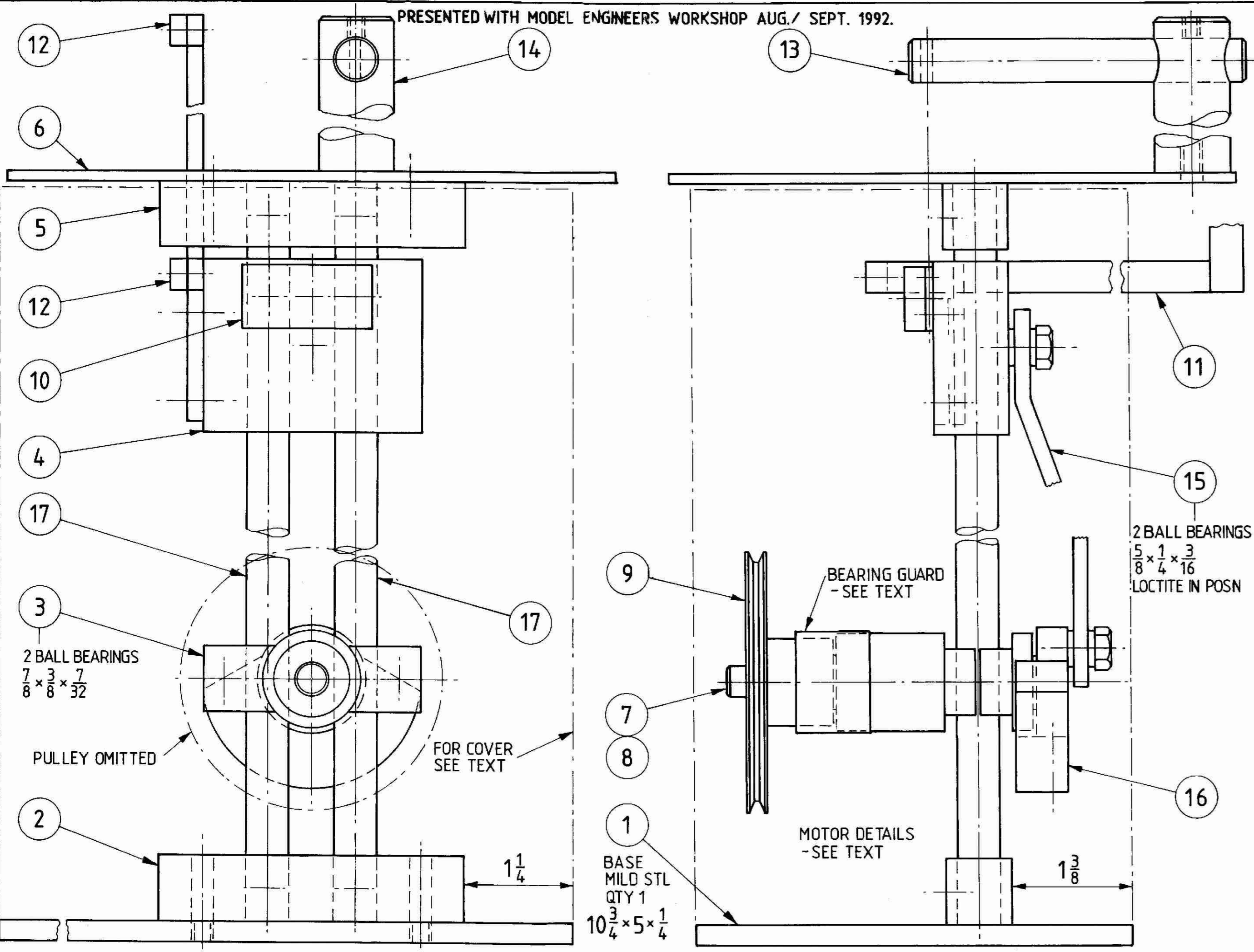
ITEM 3 BEARING HOUSING MILD STEEL QTY 1
