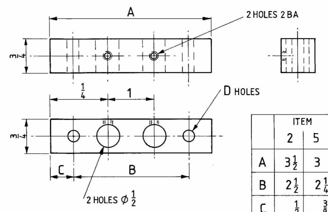
ITEMS 2 & 5 BLOCKS MILD STEEL QTY 1 EACH
