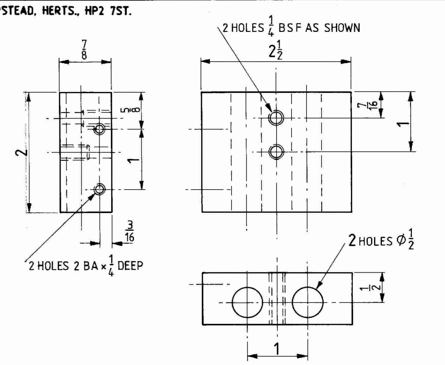
ITEM 4 TOOL BLOCK BRASS QTY 1
