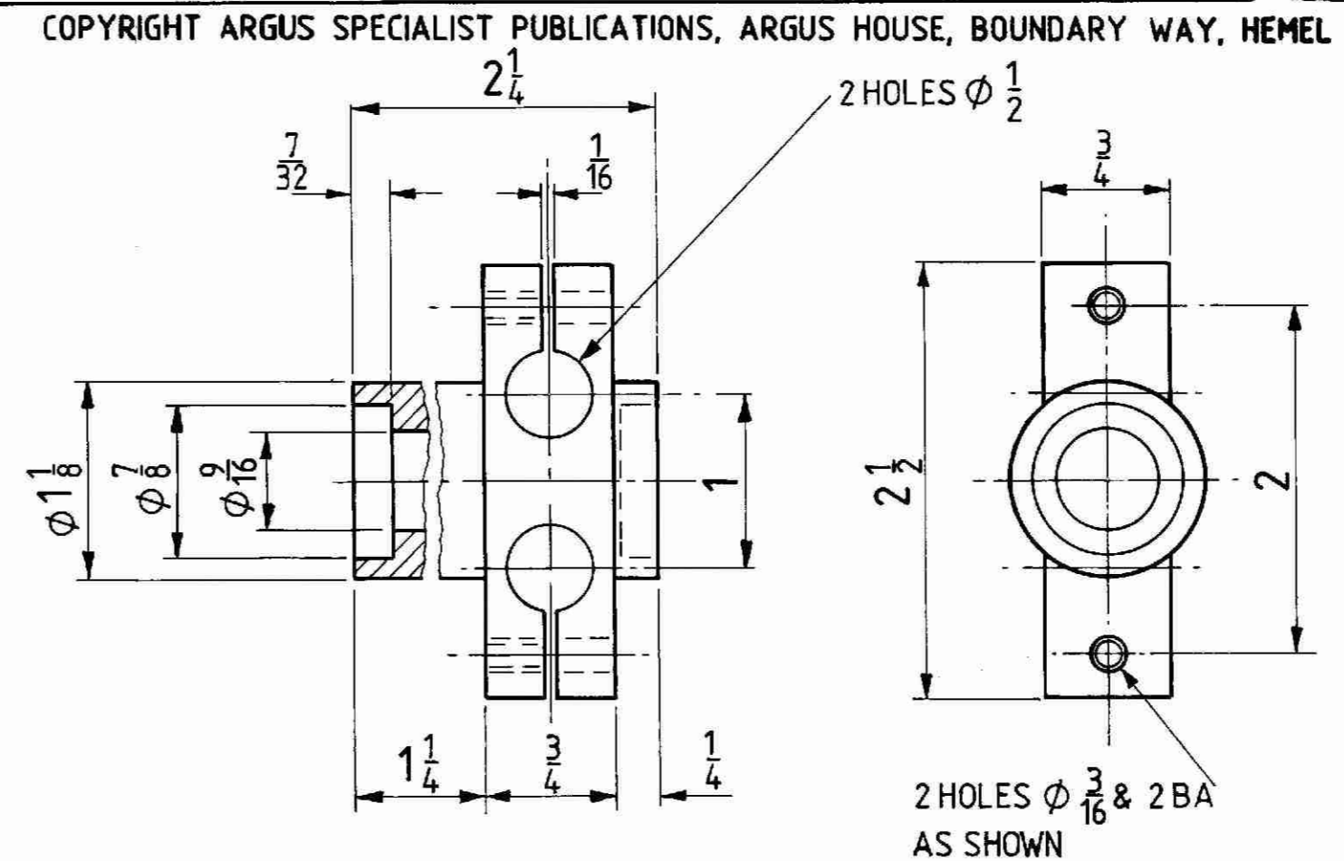
ITEM 3 BEARING HOUSING MILD STEEL QTY 1
