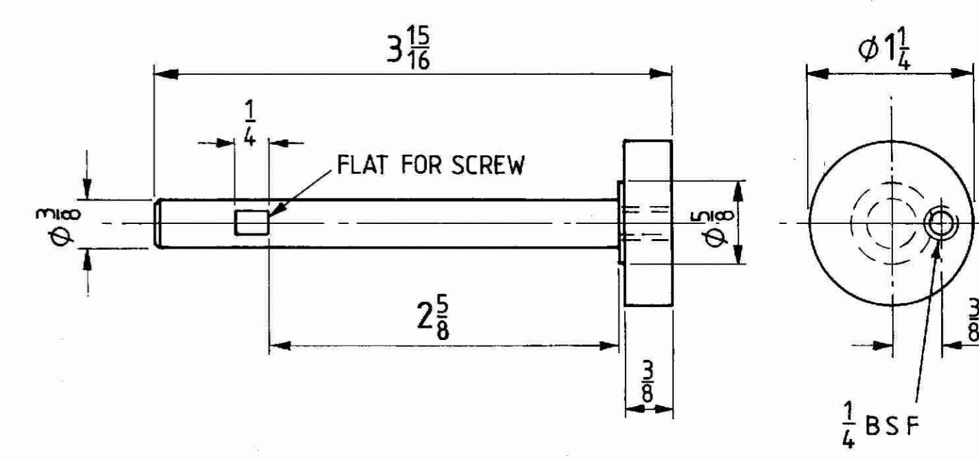
ITEM 4 TOOL BLOCK BRASS QTY 1
