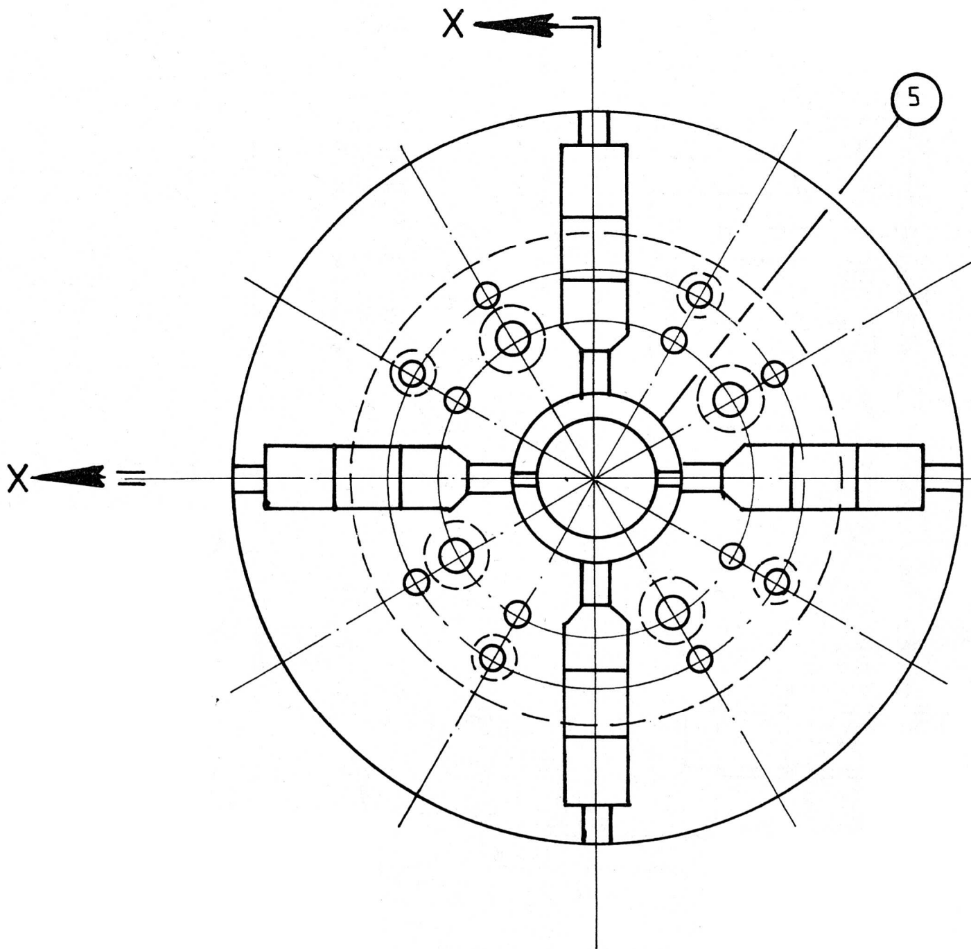
CHUCK ASSEMBLY.
