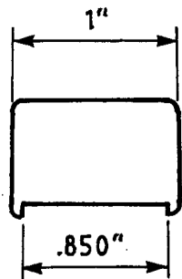
BRAKE BRACKET PAD. 1 off. - 16S.W.G. M.S.
