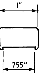
MOVING ARM BRAKE PAD. 2 off. - 16S.W.G. M.S.
