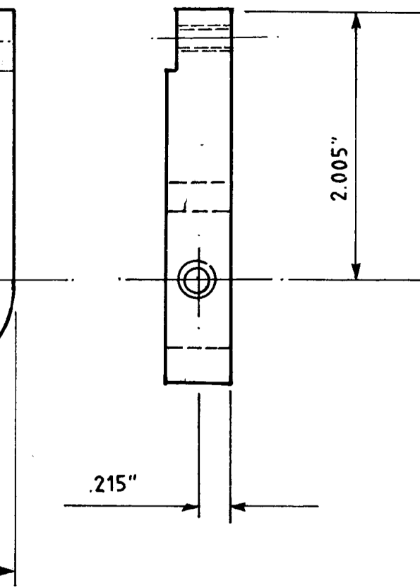
(SETTING)-HARD ALUMINIUM. OTHER DETAILS AS MOVING ARM.
