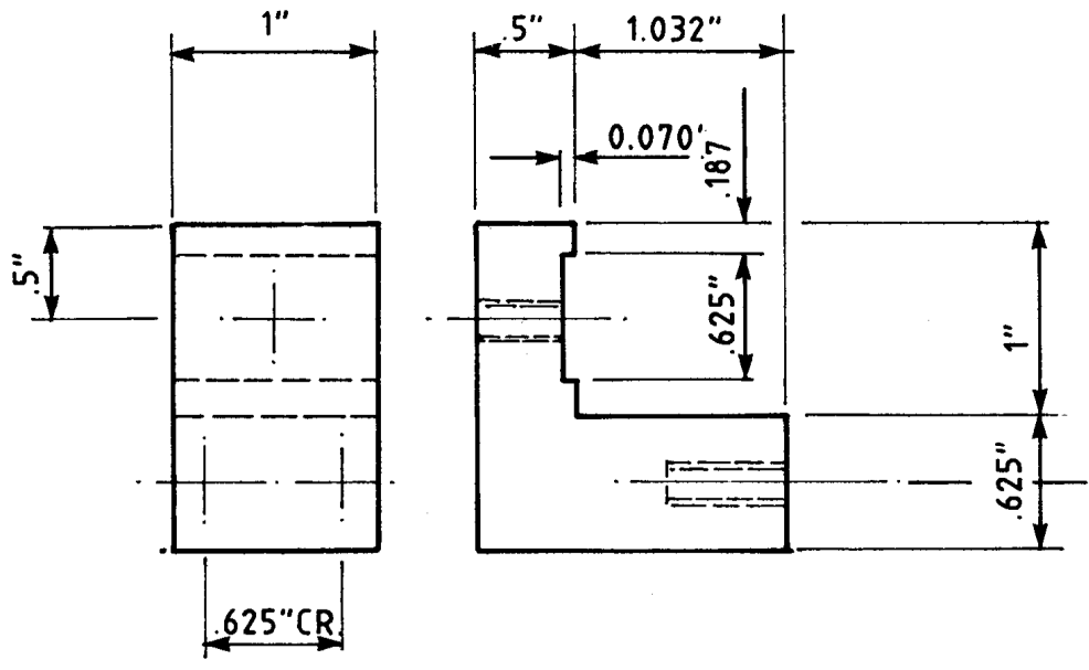
BRAKE BRACKET
