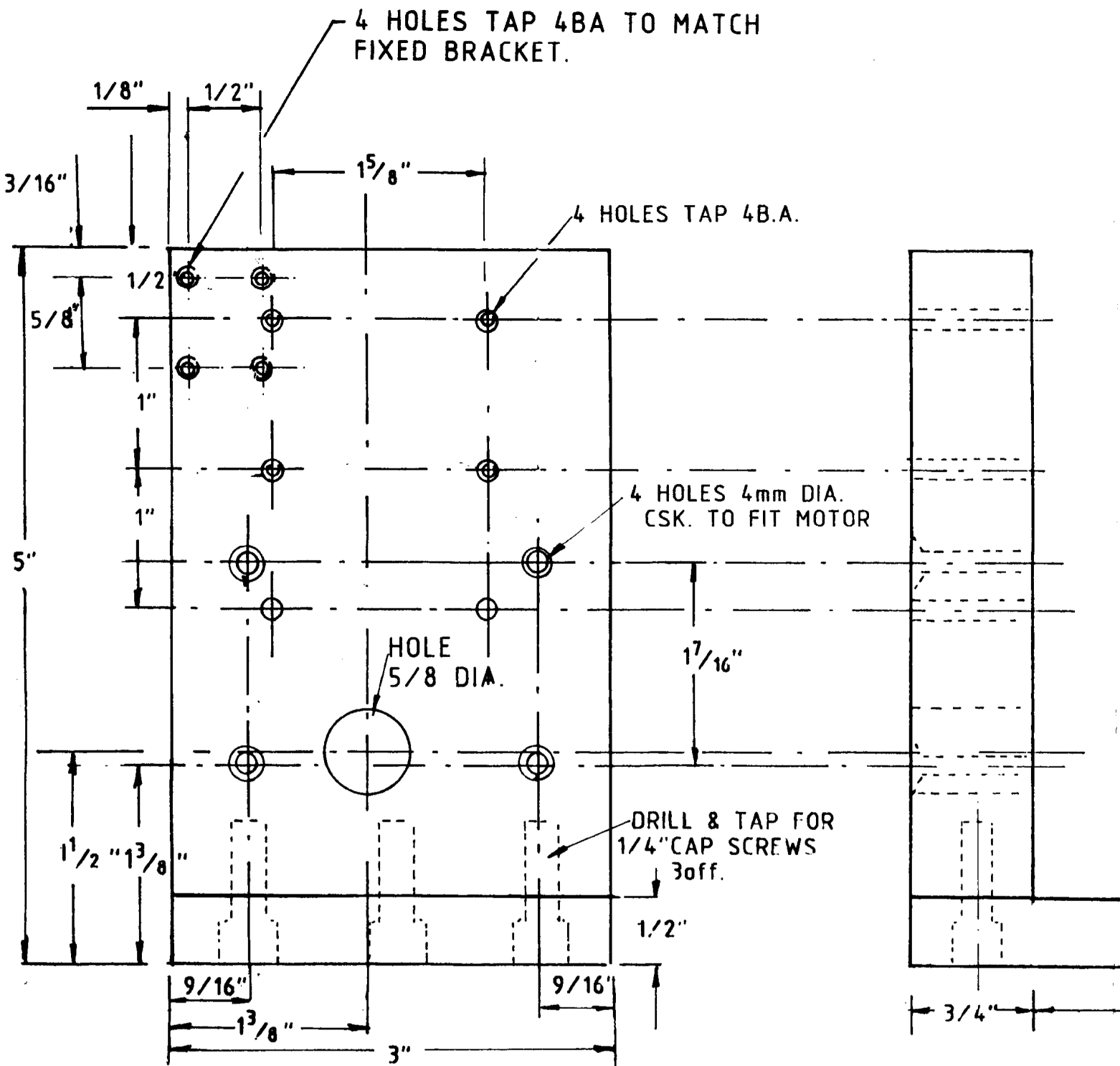
FRAME OR BODY 1off. -MATL. M/STEEL.
