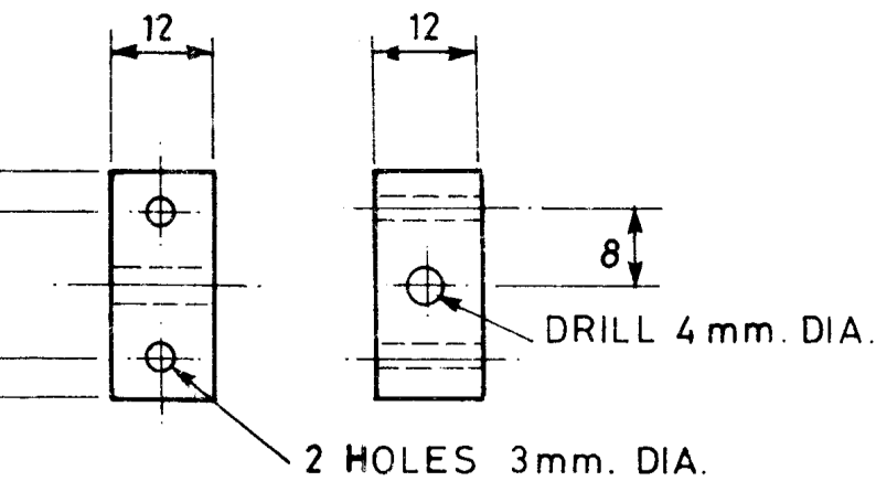
BEARING BLOCK 2 off BRASS
