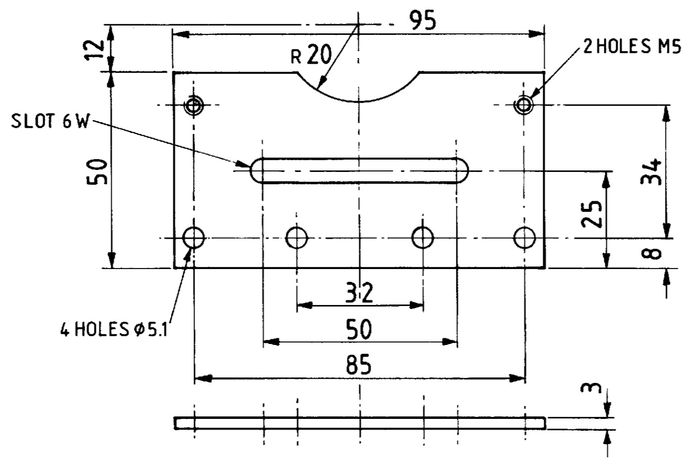
ITEM 3 FIXED PLATE MILD STEEL QTY 1
