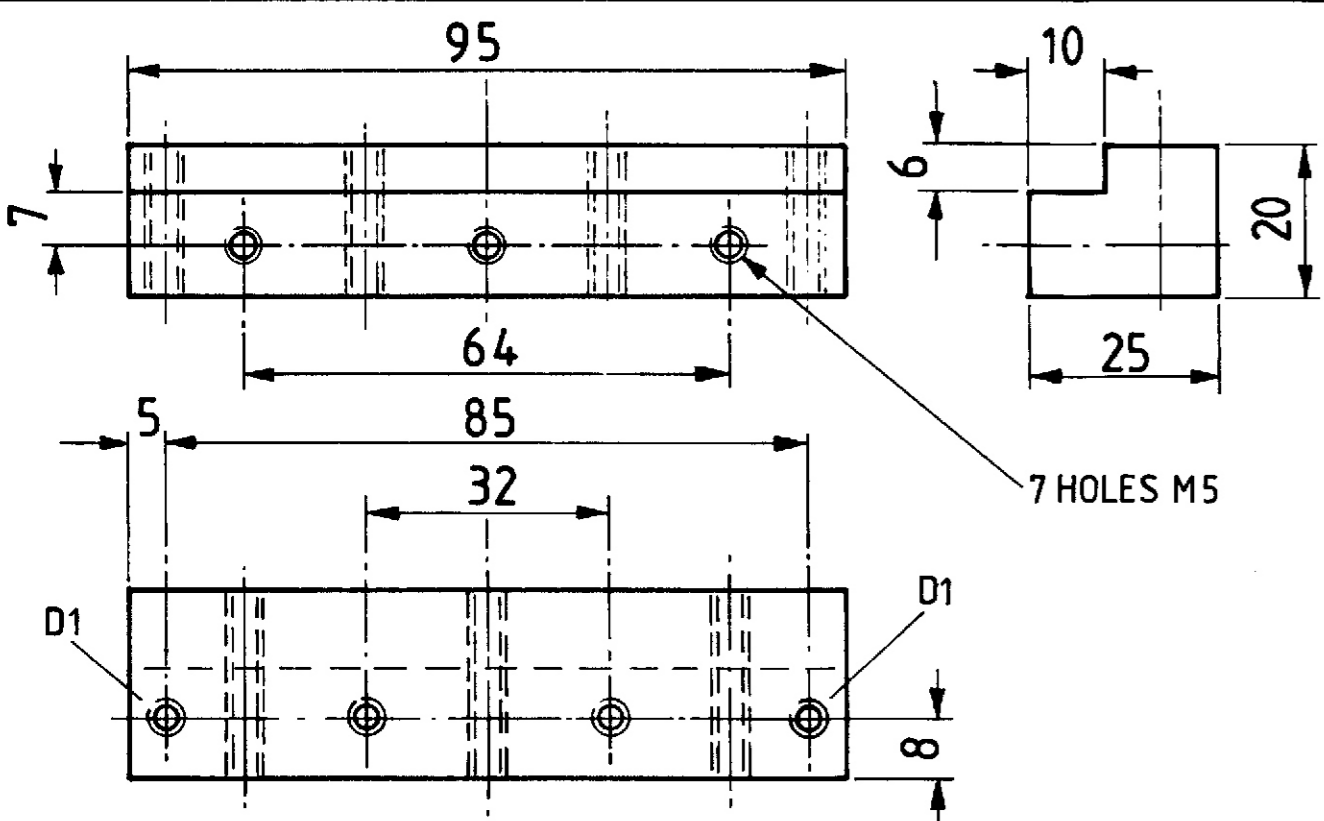
ITEM 2 BUTTRESS MILD STEEL QTY 1
