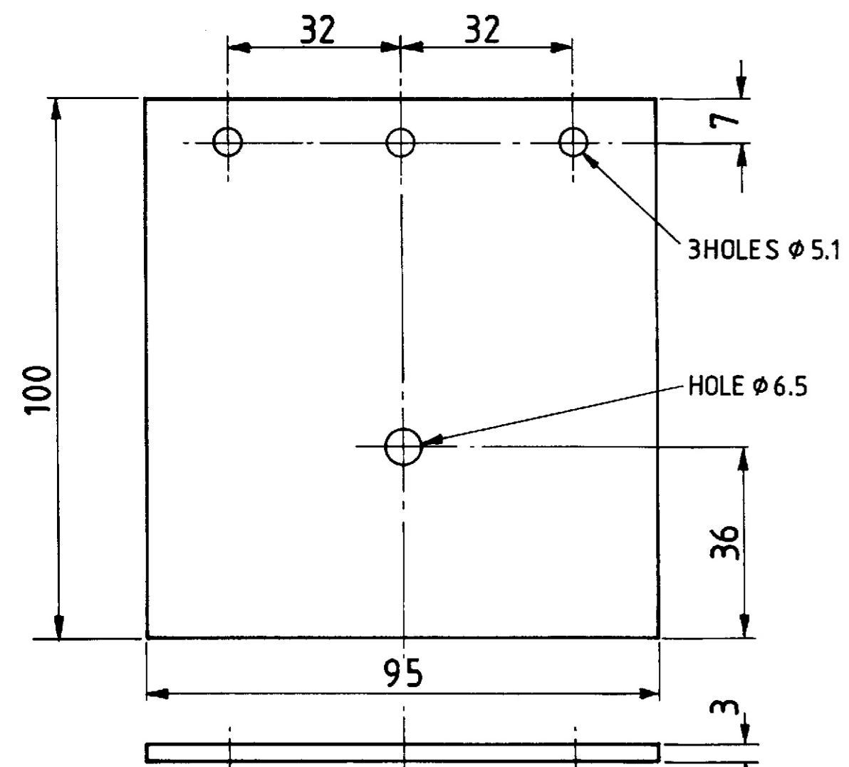
ITEM 1 BASE PLATE MILD STEEL QTY 1
