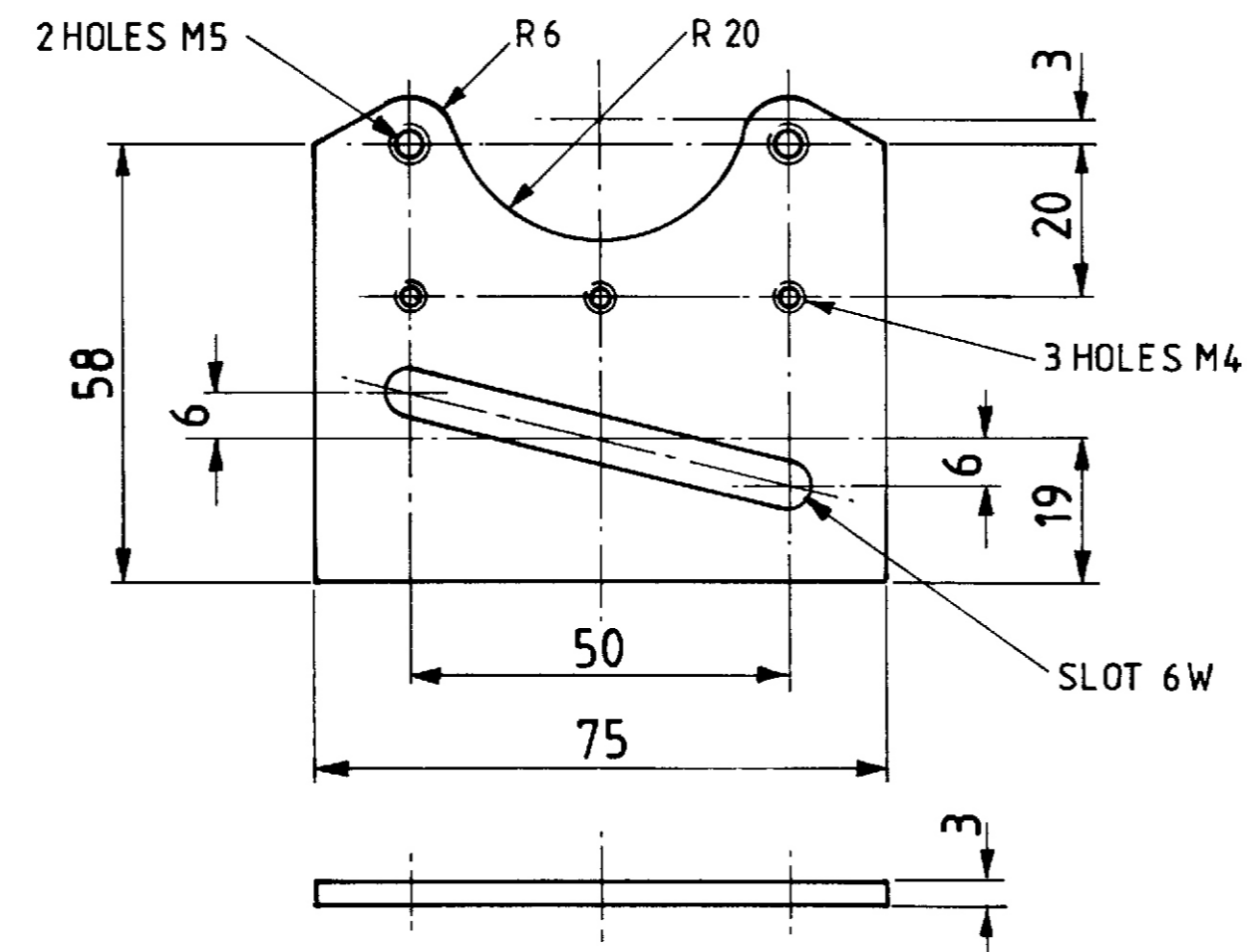
ITEM 4 SLIDE PLATE MILD STEEL QTY 1
