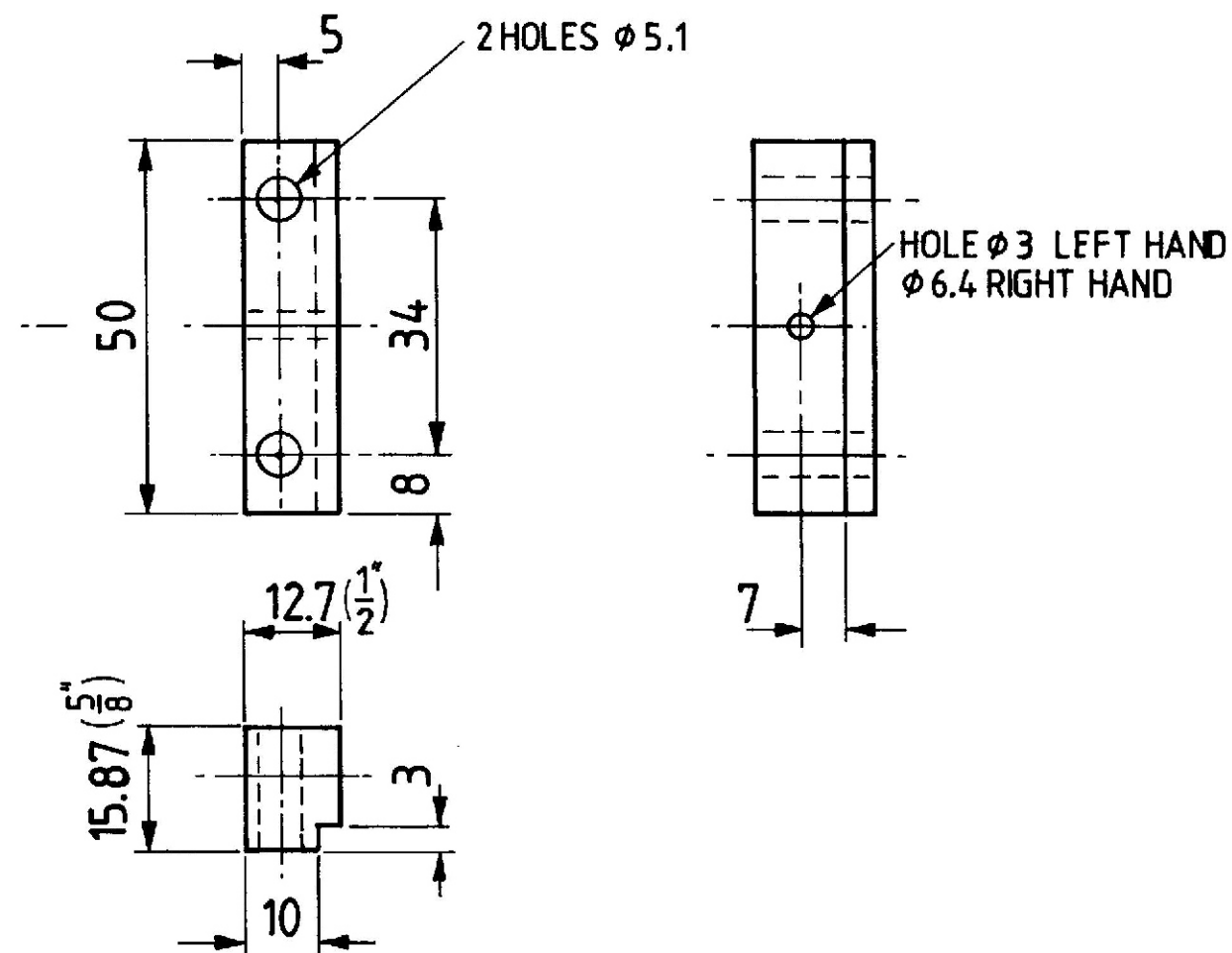
ITEM 5 SUPPORT PLATE MILD STEEL QTY 1
