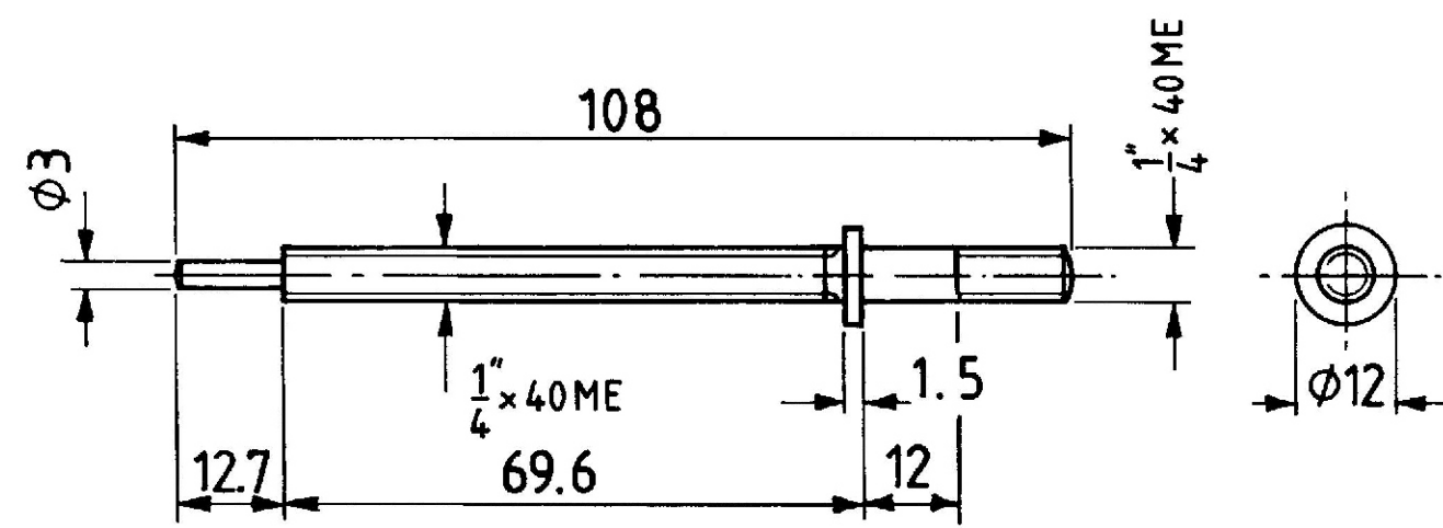
ITEM 8 ADJUSTING SHAFT MILD STEEL QTY 1
