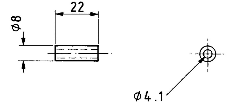
ITEM 13 SUPPORT SPACER MILD STEEL QTY 3
