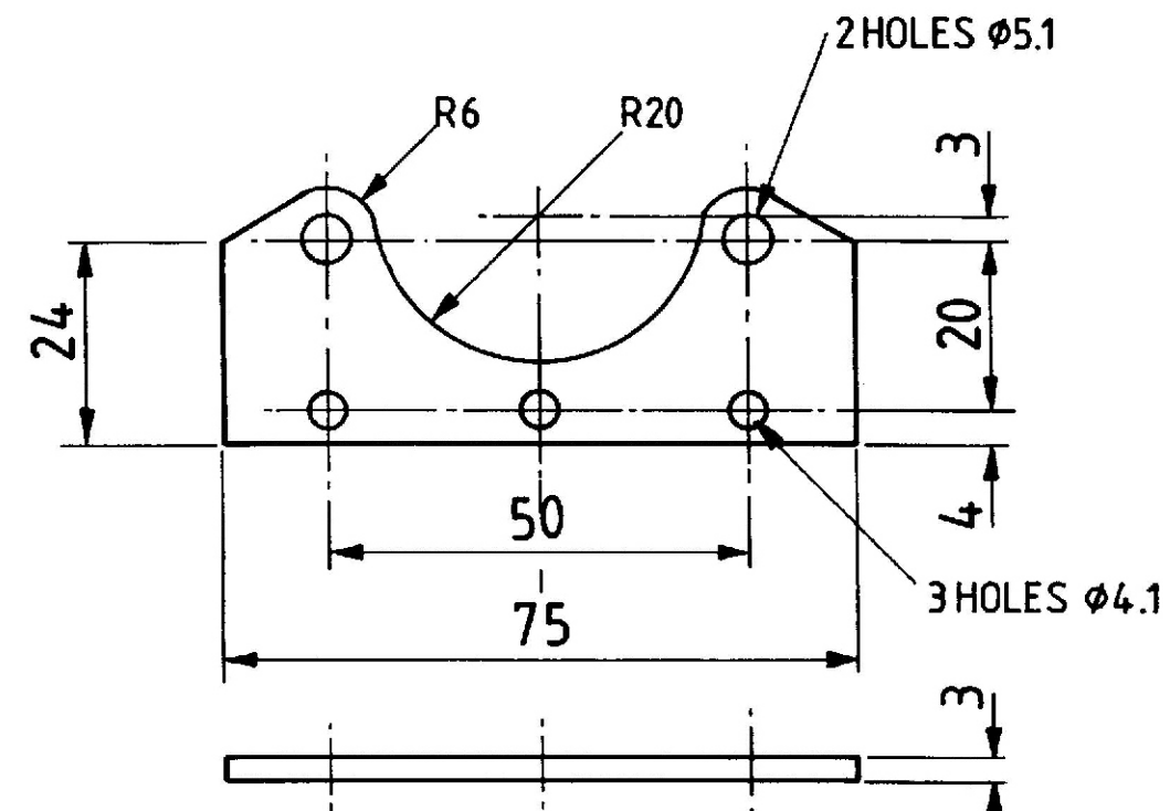
ITEM 5 SUPPORT PLATE MILD STEEL QTY 1
