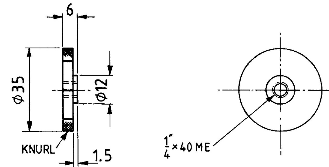
ITEM 9 ADJUSTING WHEEL MILD STEEL QTY 1
