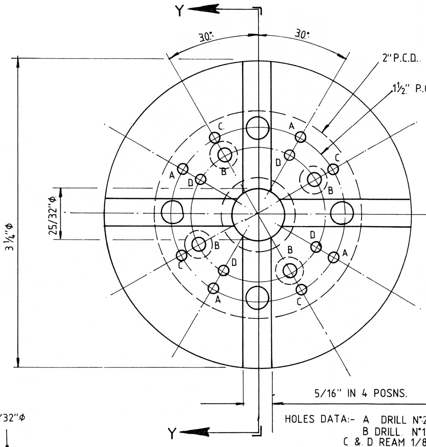
Fig.2. CHUCK BODY. (1) CAST IRON.
