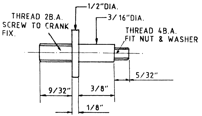
CRANK PIN 1off SCALE 2:1
